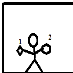
Figure 1: An observer in the lift
