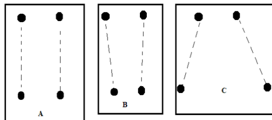
Figure 2. Two balls falling side by side in a real gravitational field
